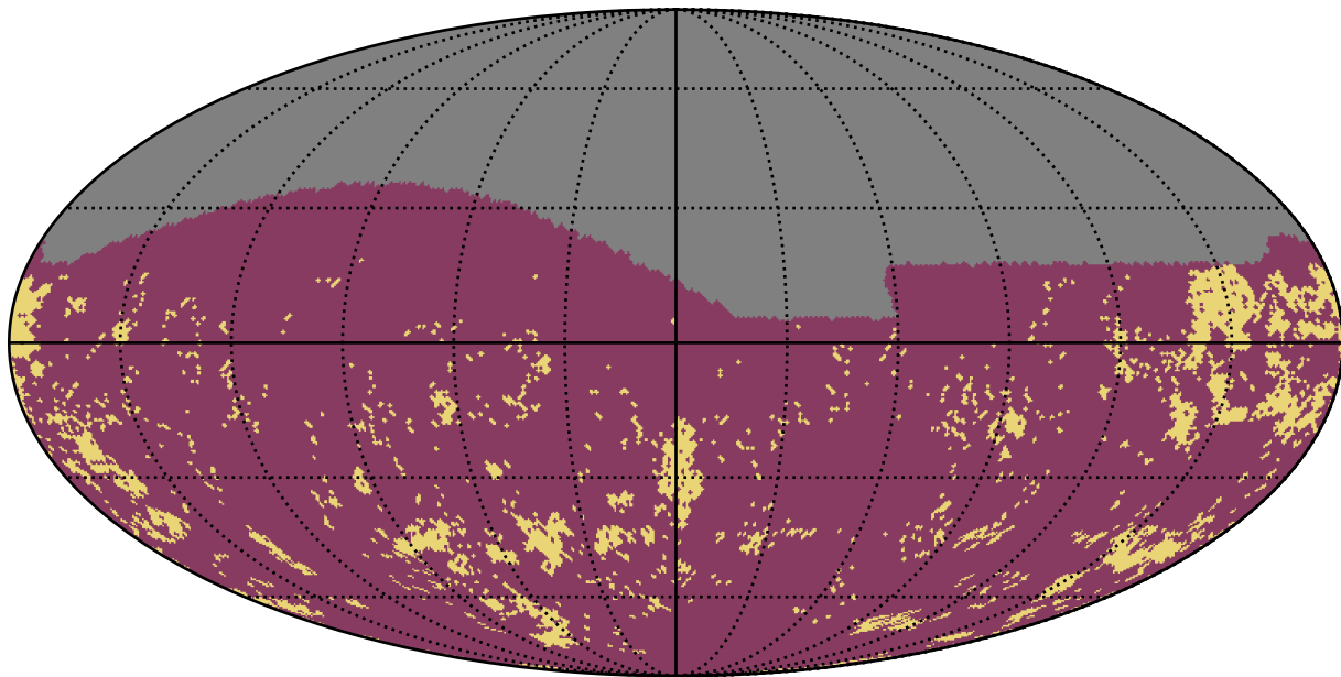
weather_cloudso14v3.4_10yrs g band: Gaps_3hr
