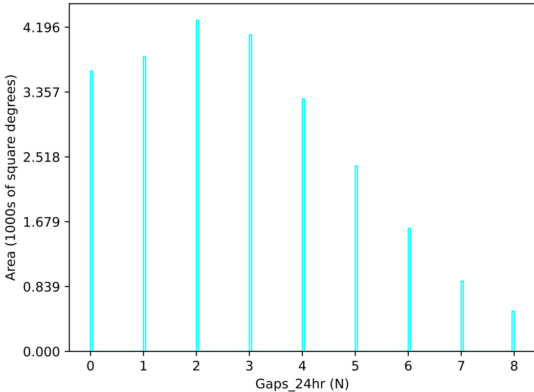
weather_cloudso14v3.4_10yrs u band: Gaps_24hr
