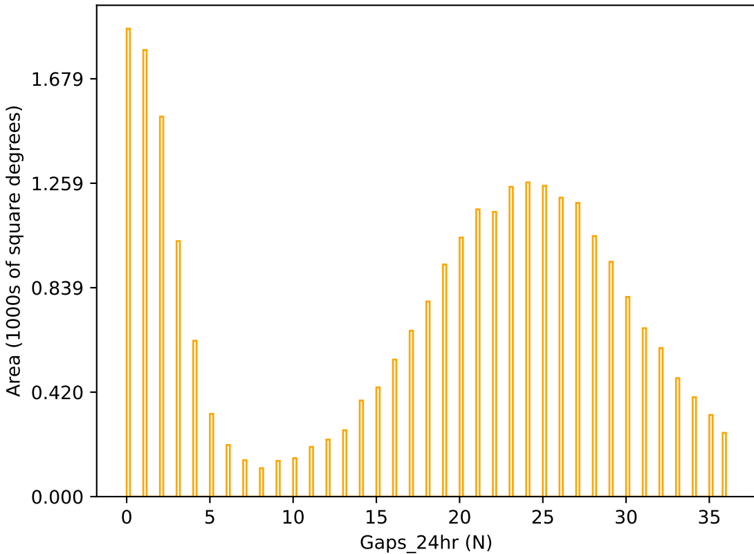
weather_cloudso14v3.4_10yrs r band: Gaps_24hr
