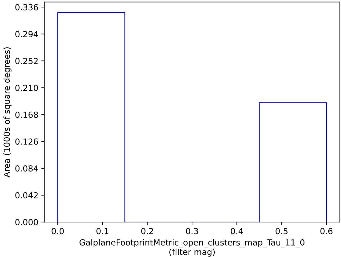
weather_cloudso14v3.4_10yrs : GalplaneFootprintMetric_open_clusters_map_Tau_11_0
