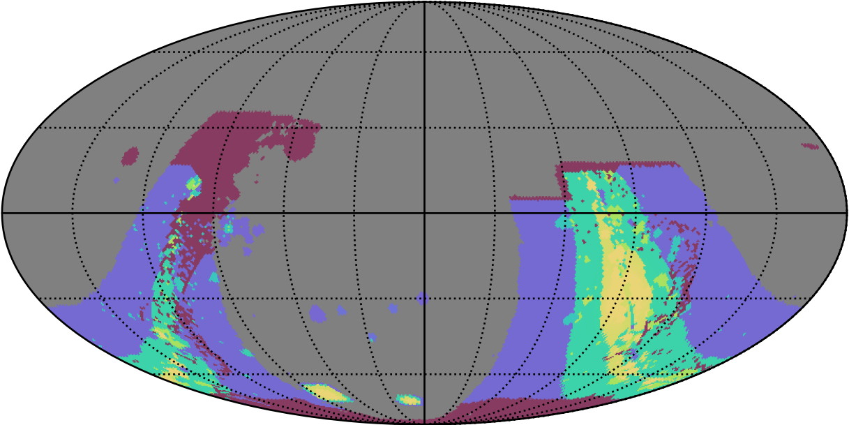
weather_cloudso14v3.4_10yrs : GalplaneFootprintMetric_combined_map_Tau_20_0
