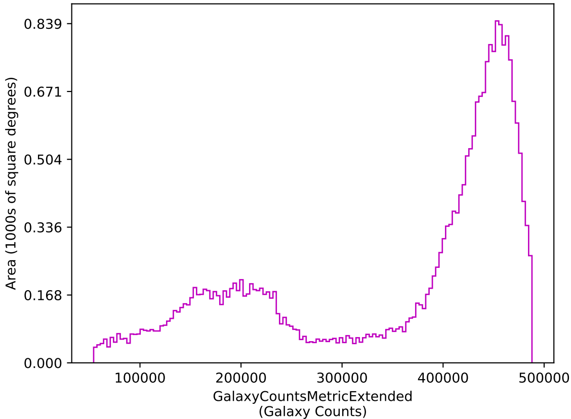
weather_cloudso14v3.4_10yrs z: GalaxyCountsMetricExtended
