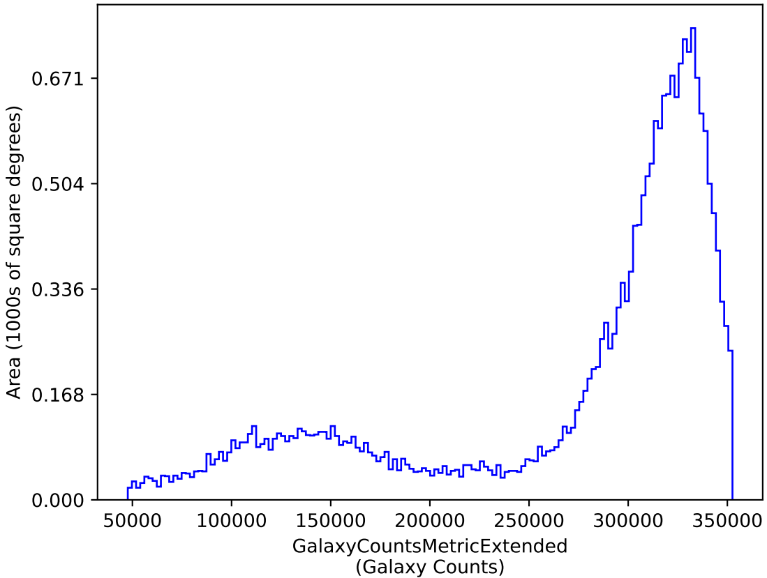
weather_cloudso14v3.4_10yrs y: GalaxyCountsMetricExtended
