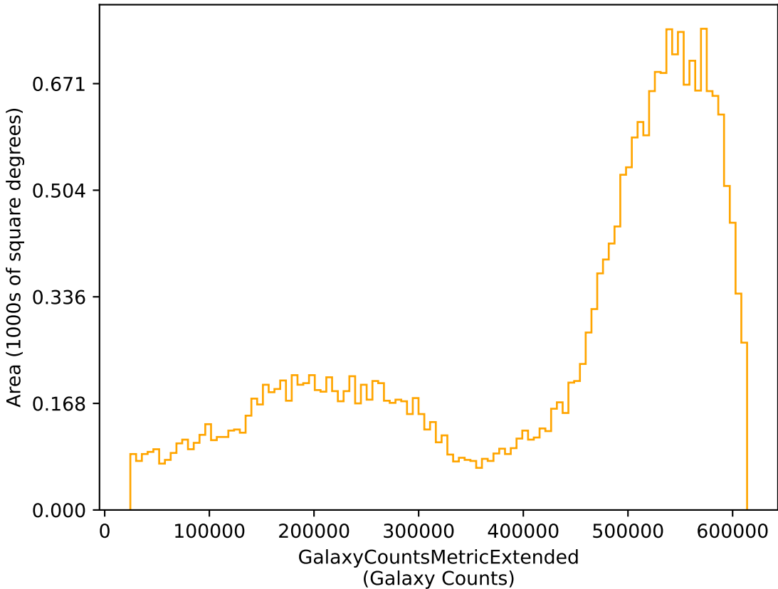
weather_cloudso14v3.4_10yrs r: GalaxyCountsMetricExtended
