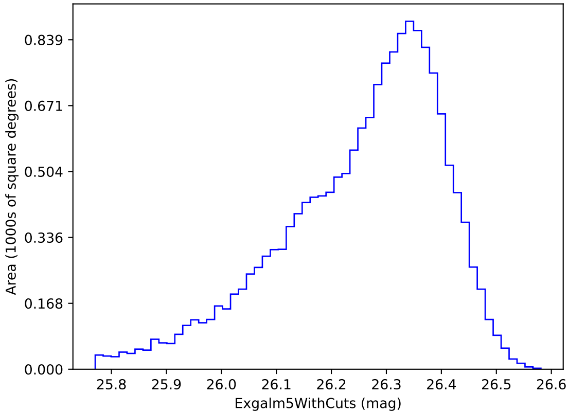
weather_cloudso14v3.4_10yrs i band non-DD year 8: ExgalM5WithCuts
