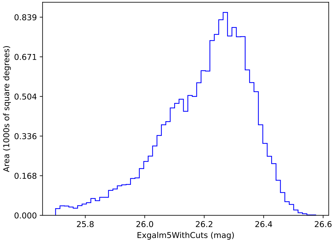
weather_cloudso14v3.4_10yrs i band non-DD year 7: ExgalM5WithCuts
