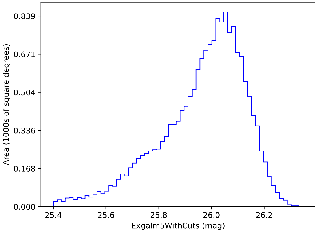
weather_cloudso14v3.4_10yrs i band non-DD year 4: ExgalM5WithCuts
