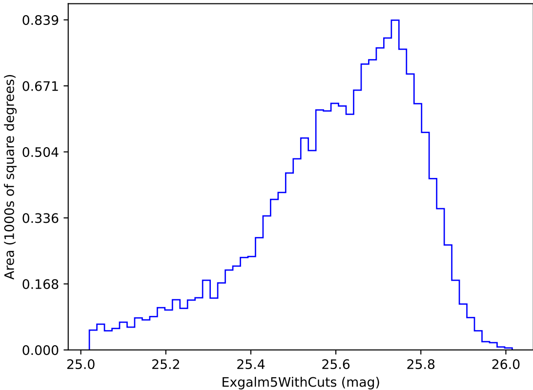
weather_cloudso14v3.4_10yrs i band non-DD year 2: ExgalM5WithCuts
