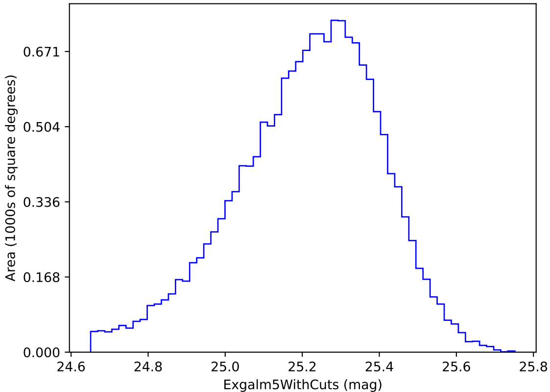
weather_cloudso14v3.4_10yrs i band non-DD year 1: ExgalM5WithCuts
