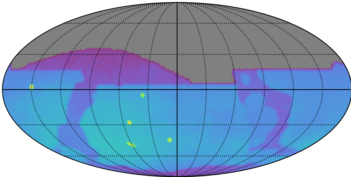
weather_cloudso14v3.4_10yrs : Brown Dwarf, L7
