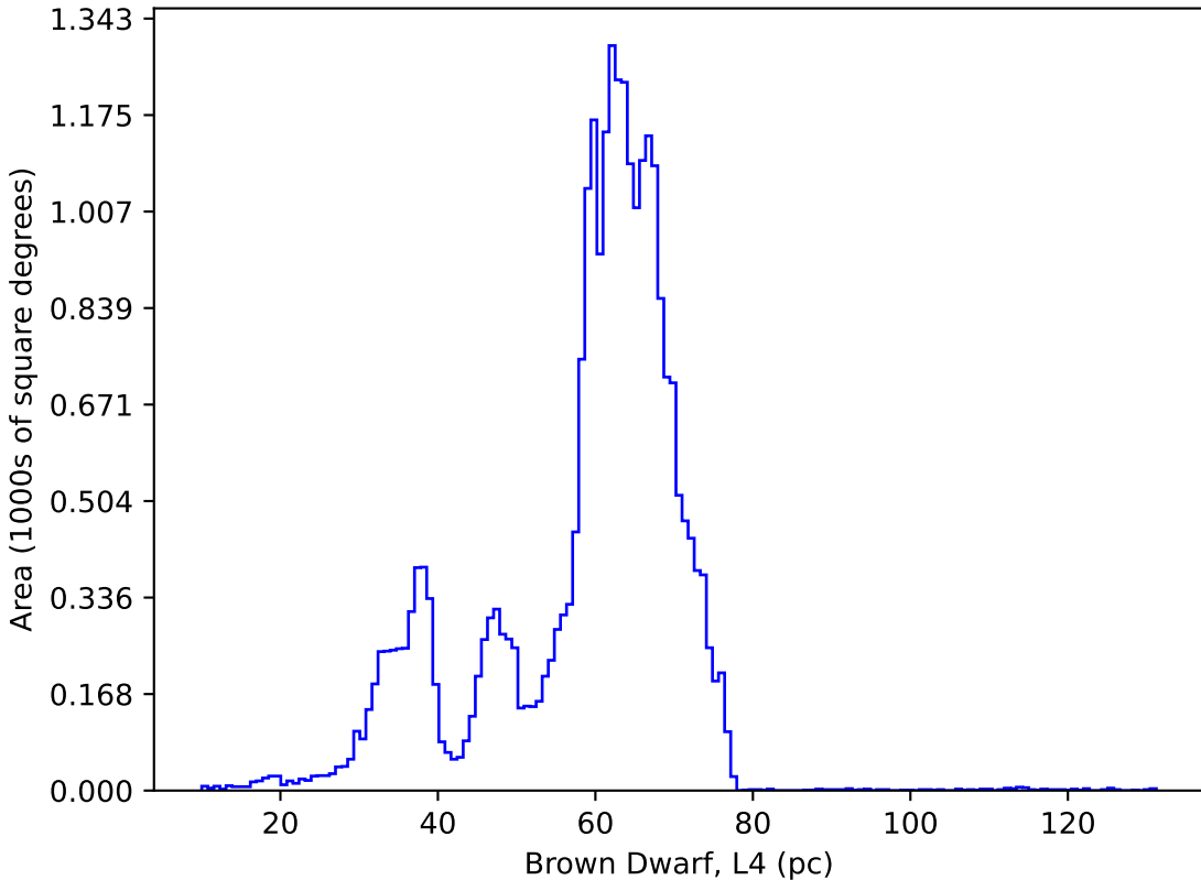
weather_cloudso14v3.4_10yrs : Brown Dwarf, L4
