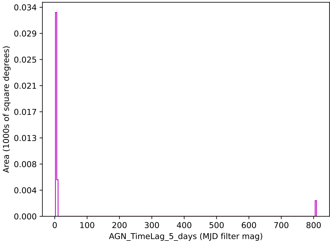
weather_cloudso14v3.4_10yrs z band: AGN_TimeLag_5_days
