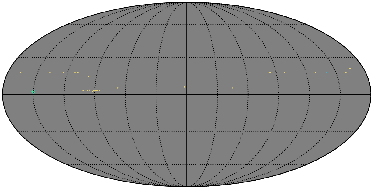
weather_cloudso14v3.4_10yrs y band: AGN_TimeLag_5_days
