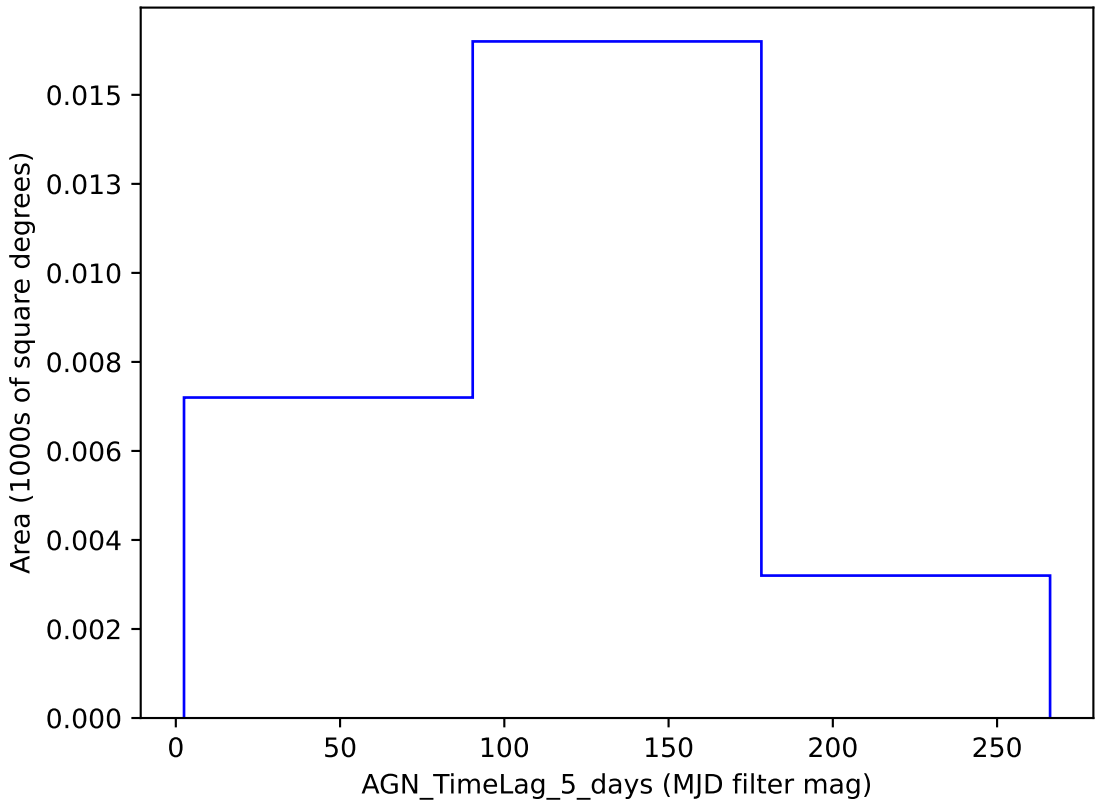
weather_cloudso14v3.4_10yrs y band: AGN_TimeLag_5_days
