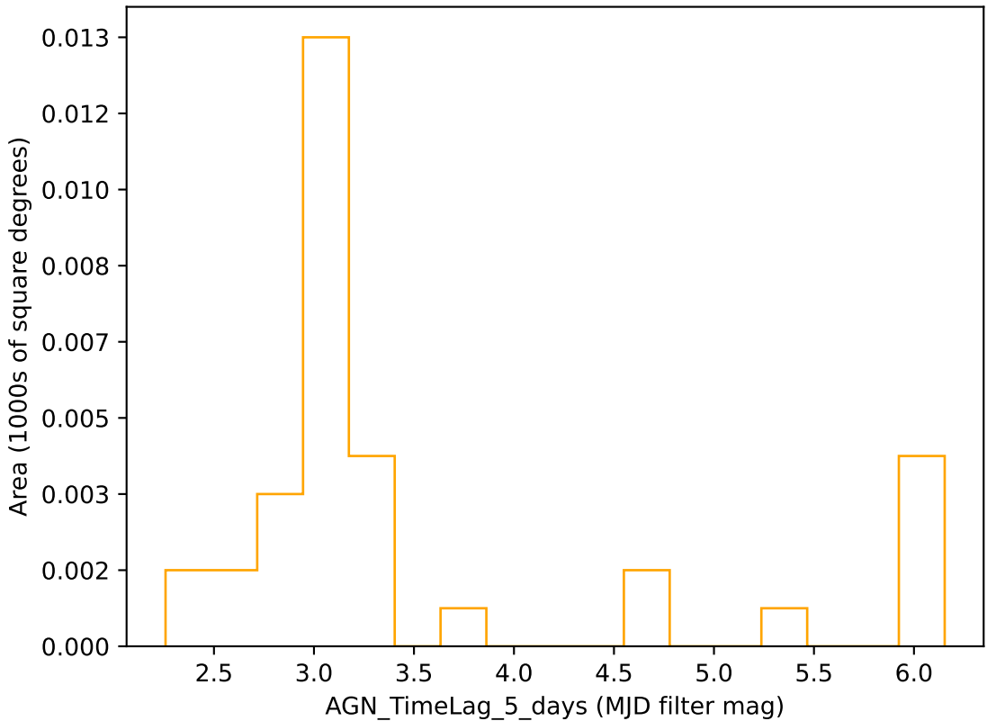
weather_cloudso14v3.4_10yrs r band: AGN_TimeLag_5_days
