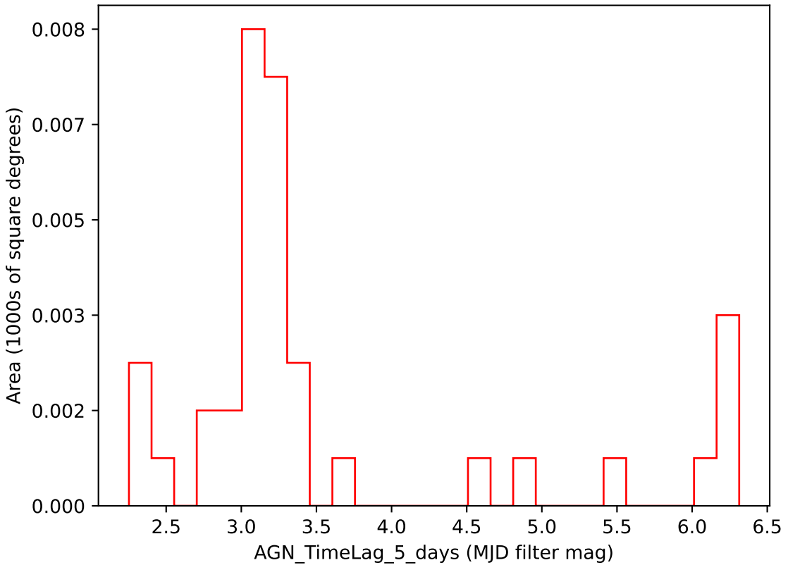
weather_cloudso14v3.4_10yrs i band: AGN_TimeLag_5_days
