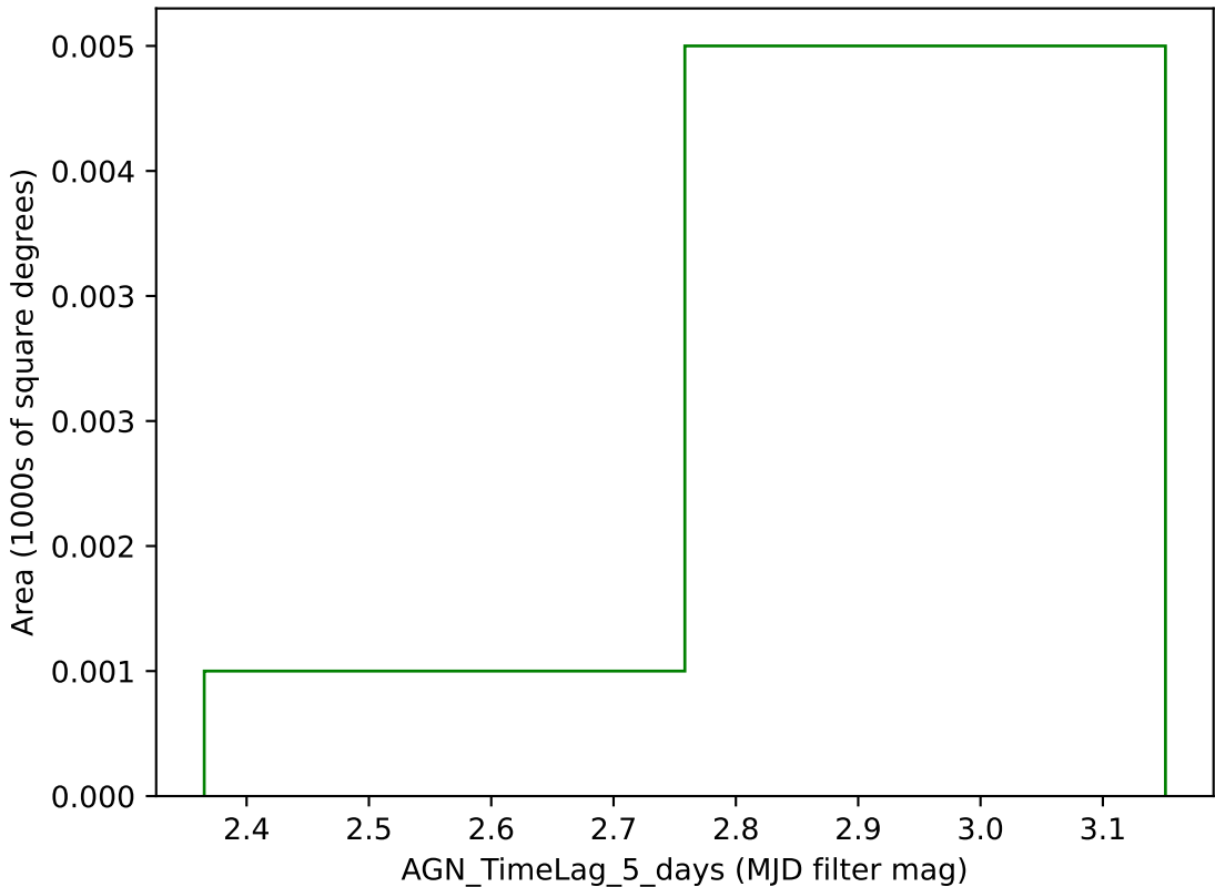
weather_cloudso14v3.4_10yrs g band: AGN_TimeLag_5_days
