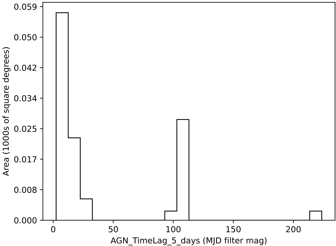
weather_cloudso14v3.4_10yrs all bands: AGN_TimeLag_5_days
