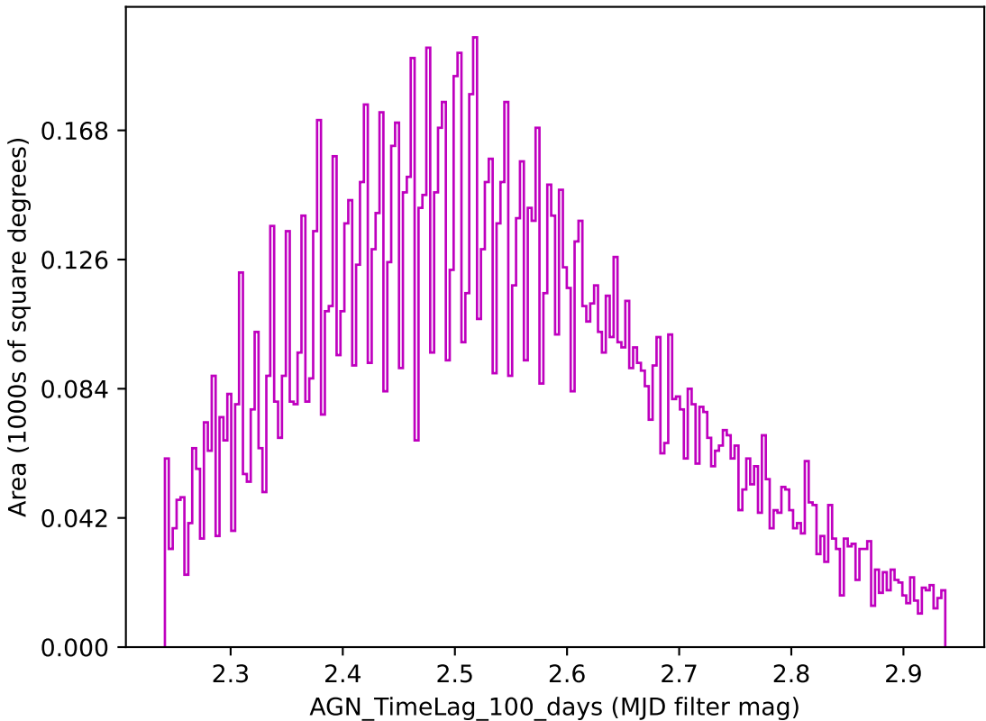
weather_cloudso14v3.4_10yrs z band: AGN_TimeLag_100_days
