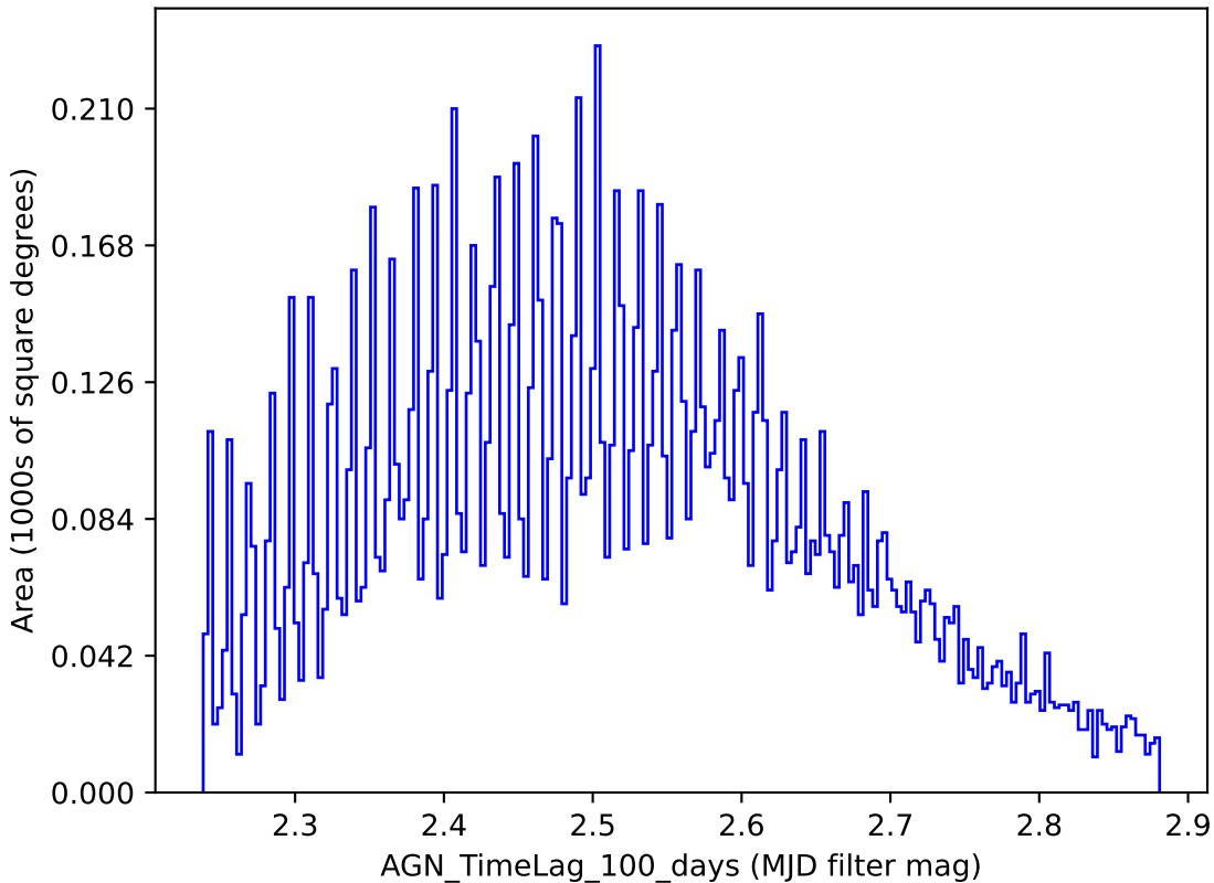
weather_cloudso14v3.4_10yrs y band: AGN_TimeLag_100_days
