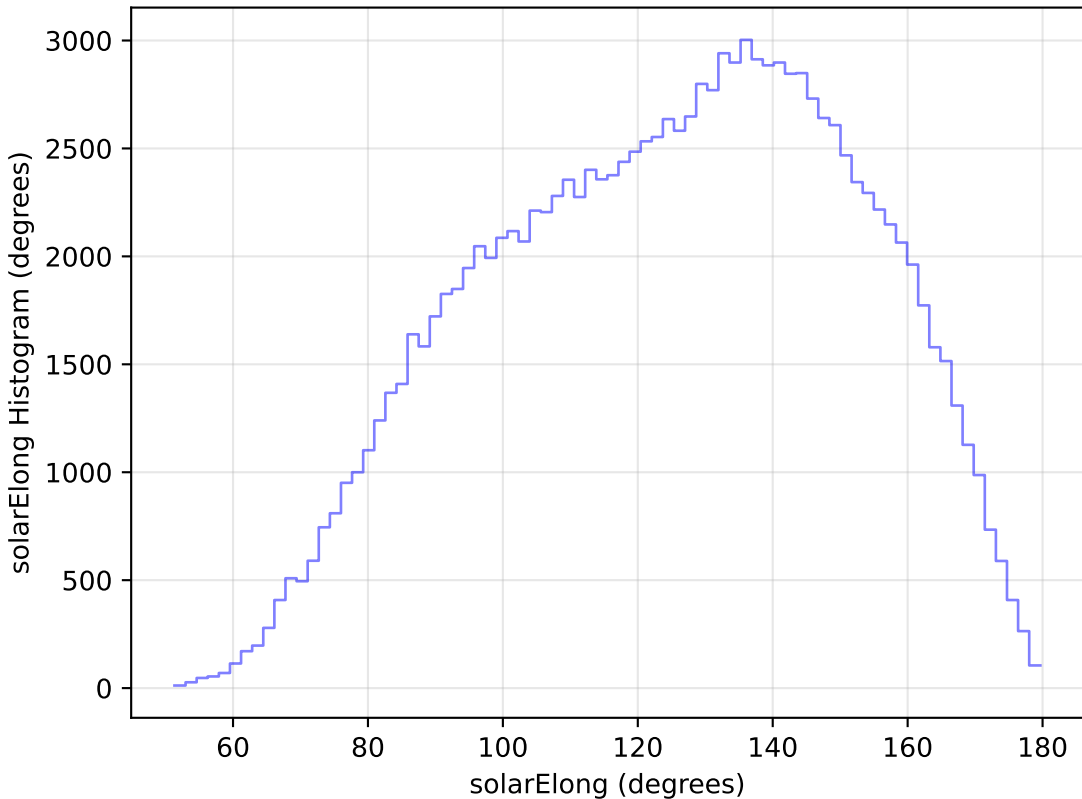
weather_cloudso14v3.4_10yrs WFD u band: solarElong Histogram
