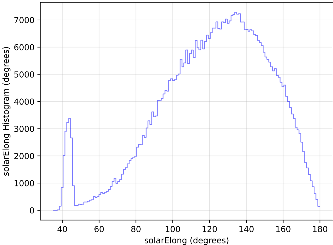
weather_cloudso14v3.4_10yrs WFD r band: solarElong Histogram
