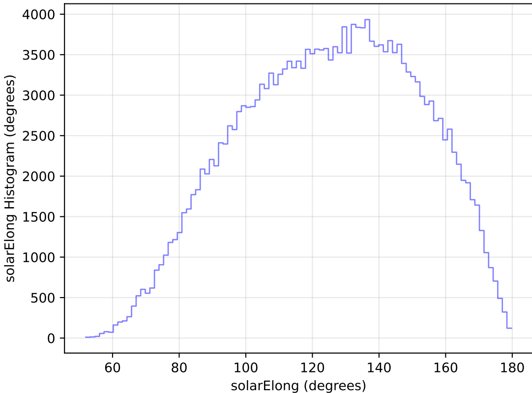
weather_cloudso14v3.4_10yrs WFD g band: solarElong Histogram
