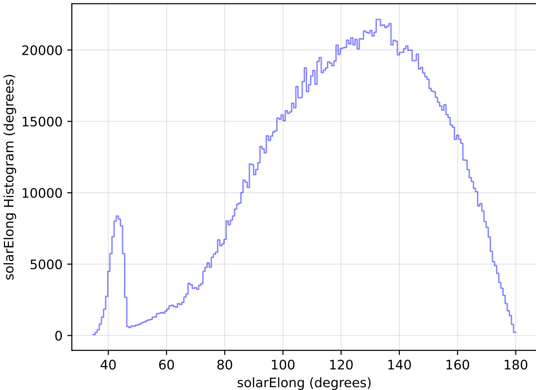
weather_cloudso14v3.4_10yrs WFD all bands: solarElong Histogram
