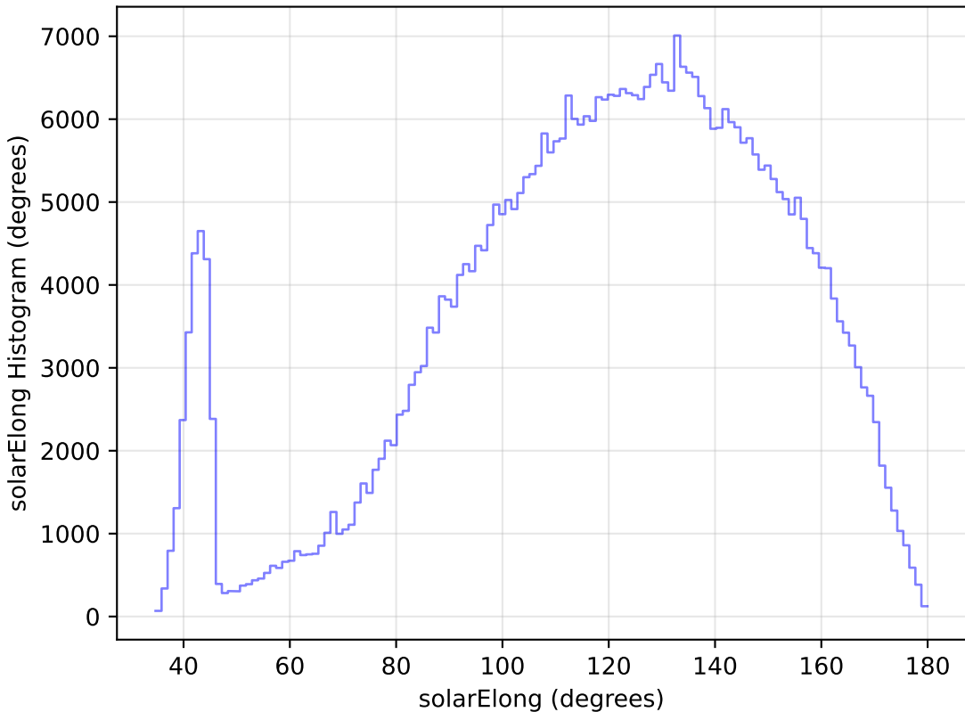
weather_cloudso14v3.4_10yrs All sky z band: solarElong Histogram
