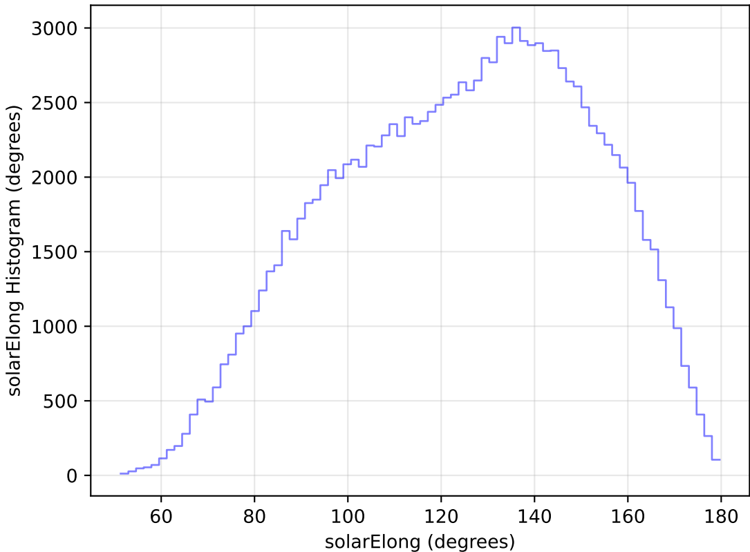
weather_cloudso14v3.4_10yrs All sky u band: solarElong Histogram
