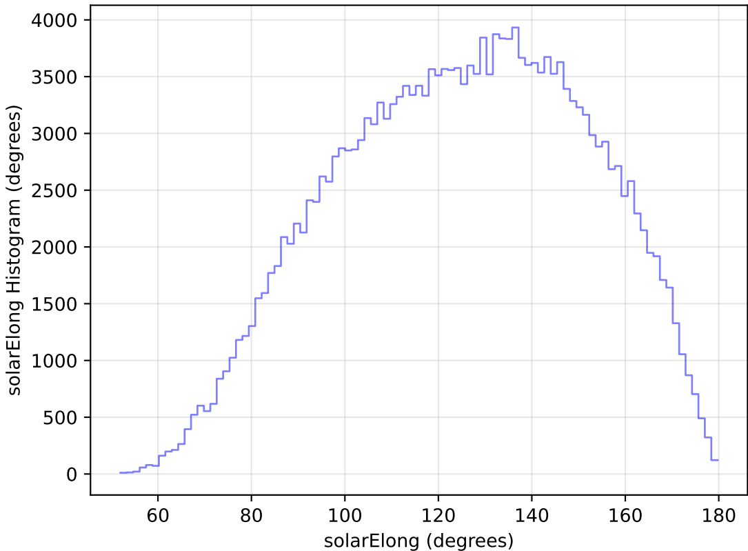
weather_cloudso14v3.4_10yrs All sky g band: solarElong Histogram
