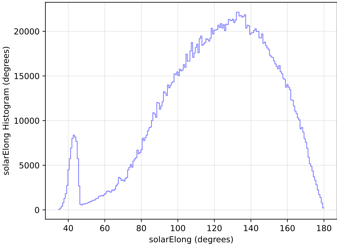
weather_cloudso14v3.4_10yrs All sky all bands: solarElong Histogram
