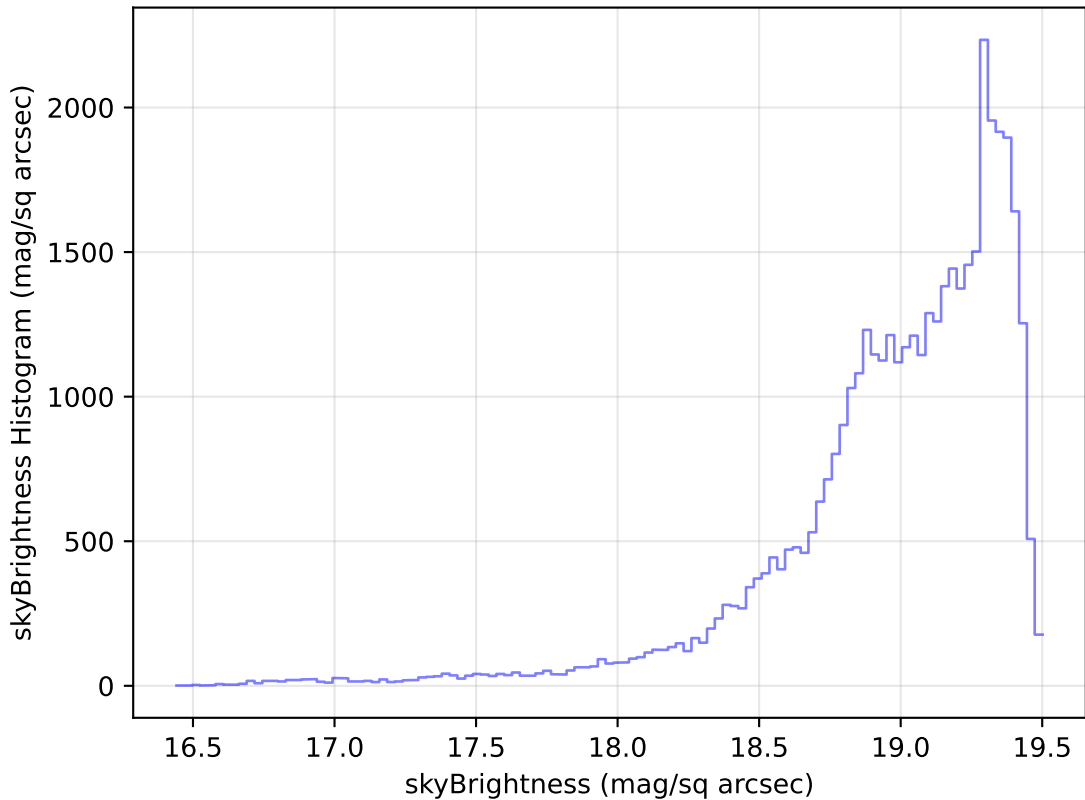
weather_cloudso14v3.4_10yrs Yr 1 z band: skyBrightness Histogram
