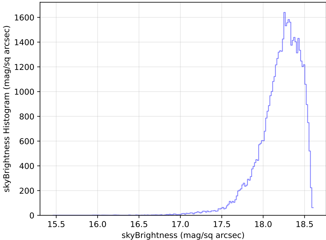
weather_cloudso14v3.4_10yrs Yr 1 y band: skyBrightness Histogram
