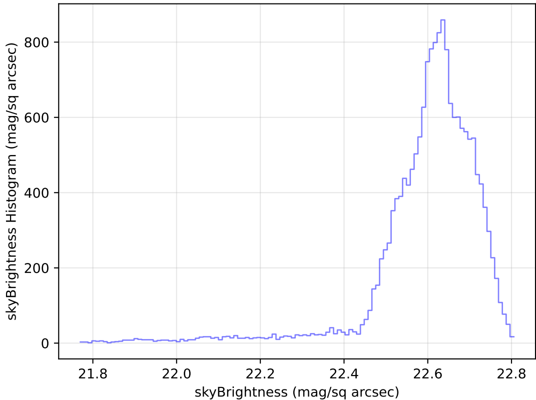
weather_cloudso14v3.4_10yrs Yr 1 u band: skyBrightness Histogram
