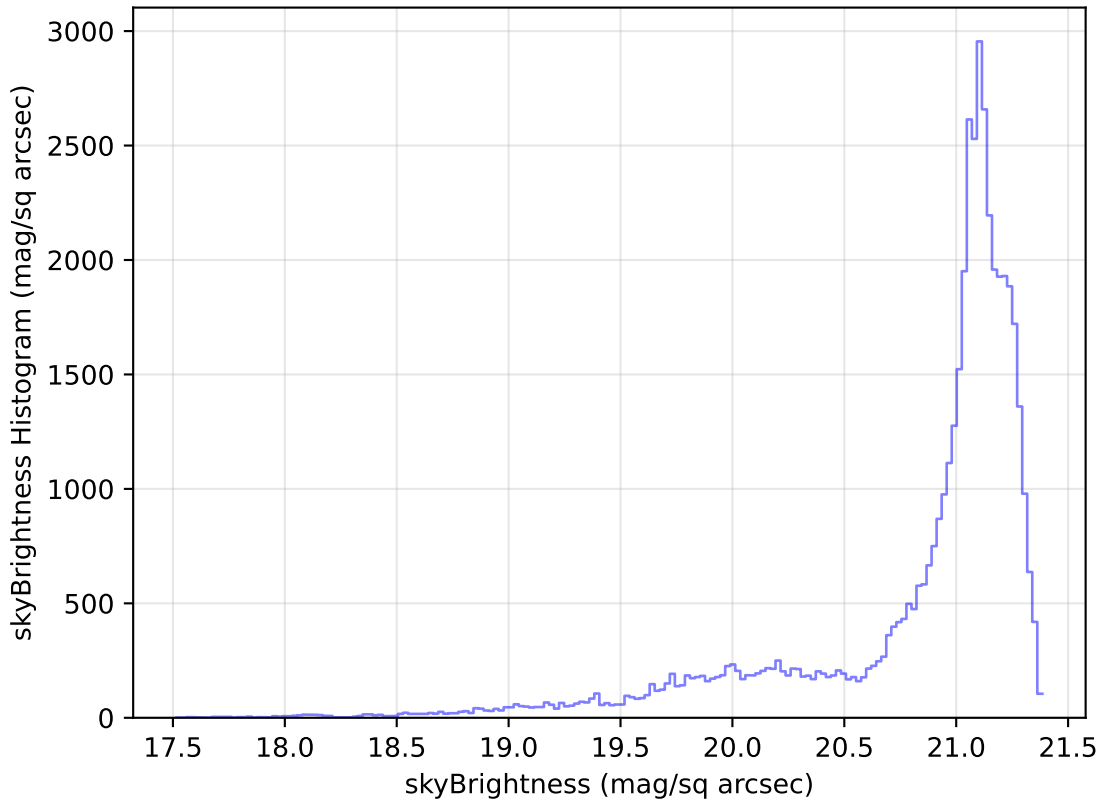
weather_cloudso14v3.4_10yrs Yr 1 r band: skyBrightness Histogram
