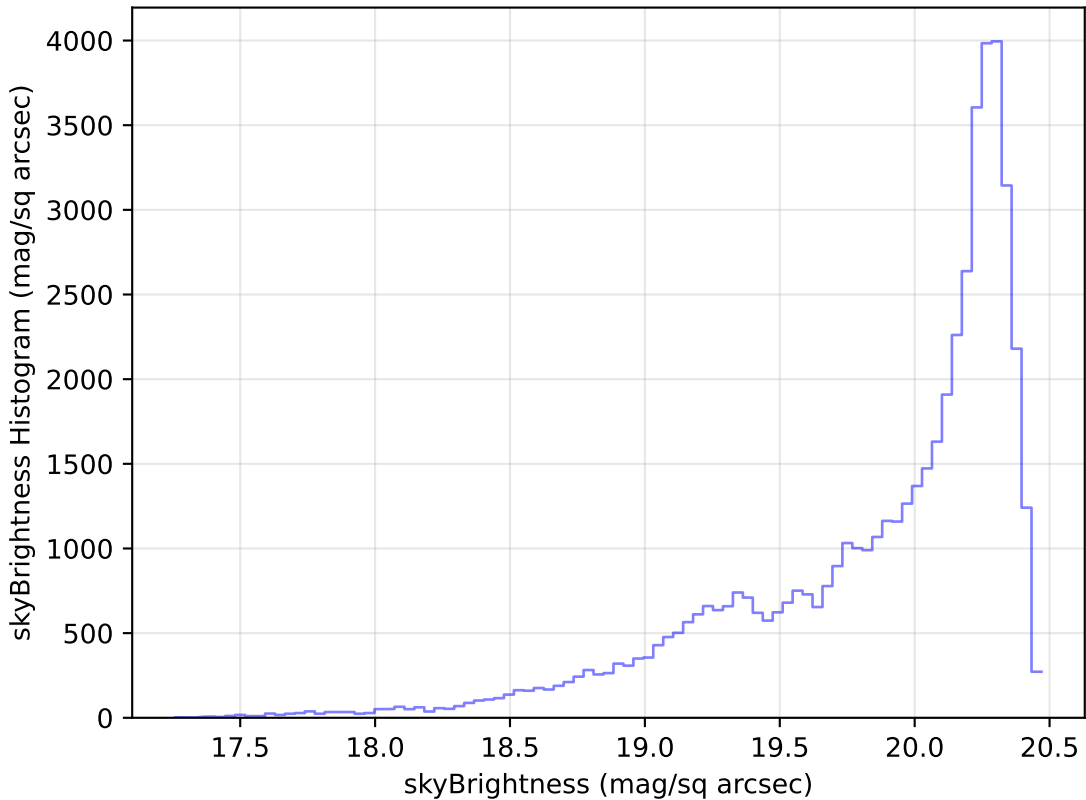
weather_cloudso14v3.4_10yrs Yr 1 i band: skyBrightness Histogram
