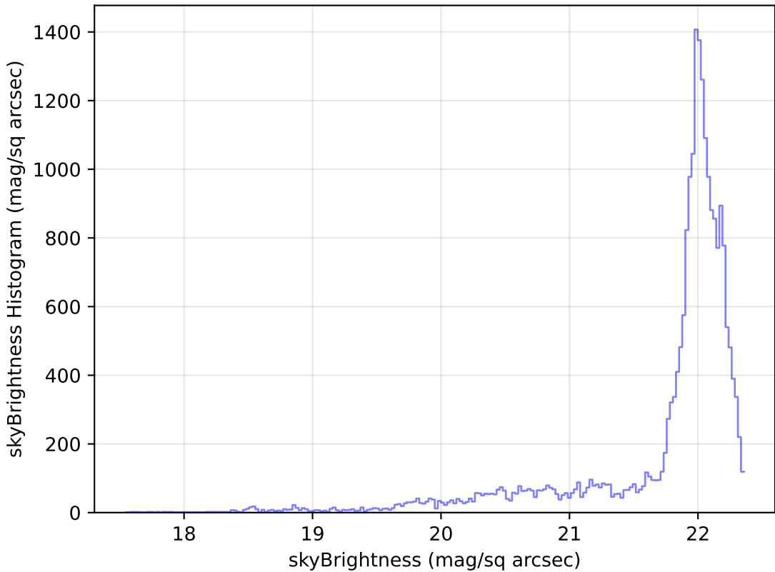
weather_cloudso14v3.4_10yrs Yr 1 g band: skyBrightness Histogram
