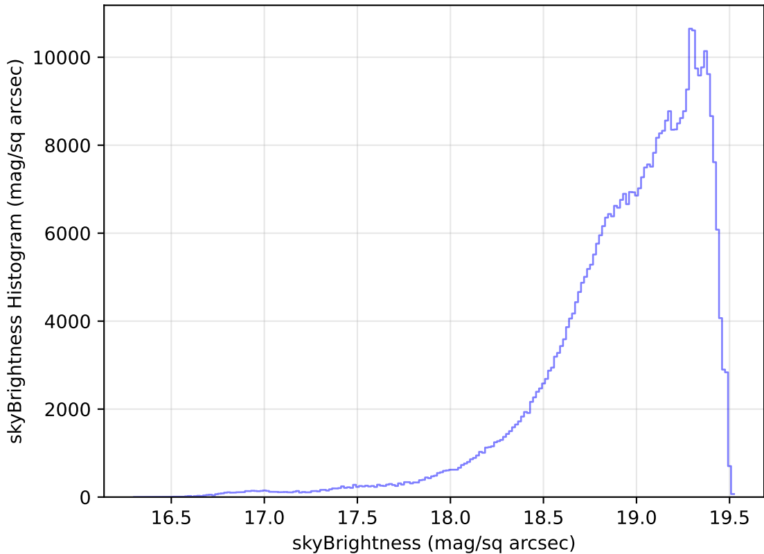
weather_cloudso14v3.4_10yrs WFD z band: skyBrightness Histogram
