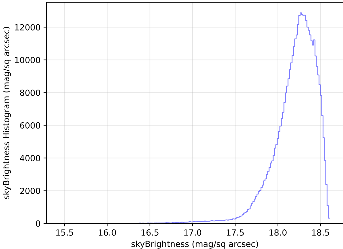
weather_cloudso14v3.4_10yrs WFD y band: skyBrightness Histogram
