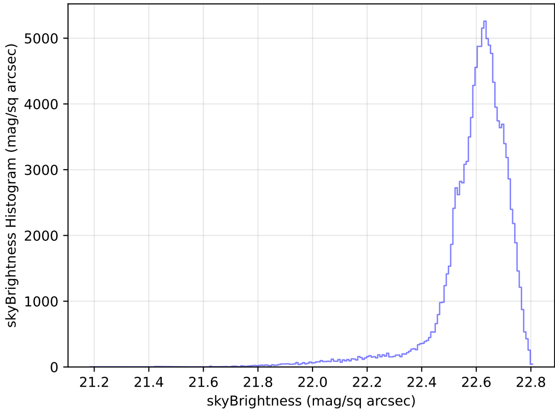
weather_cloudso14v3.4_10yrs WFD u band: skyBrightness Histogram
