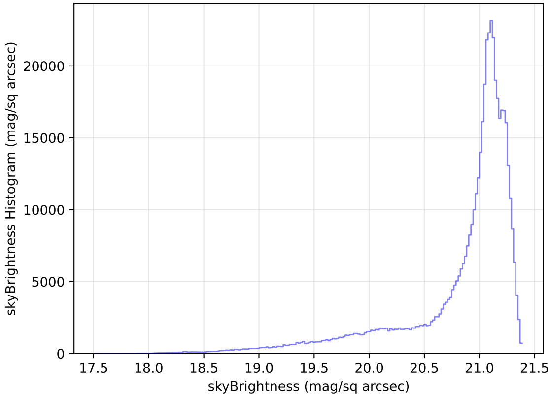
weather_cloudso14v3.4_10yrs WFD r band: skyBrightness Histogram
