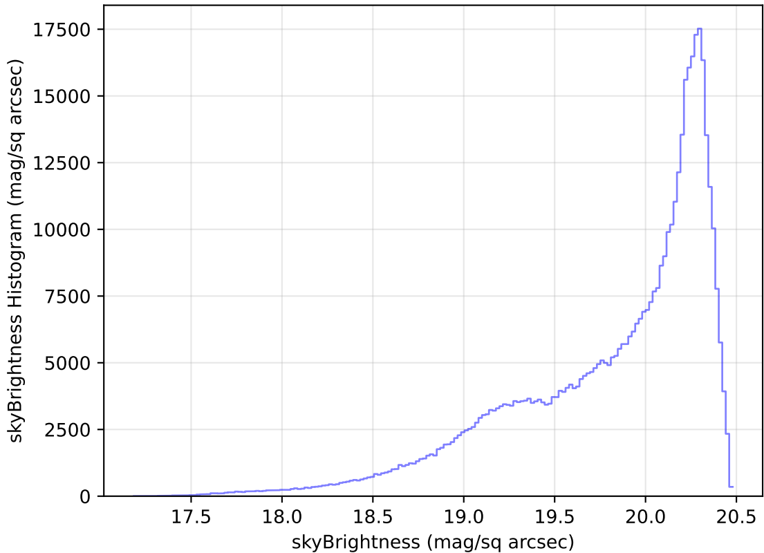
weather_cloudso14v3.4_10yrs WFD i band: skyBrightness Histogram
