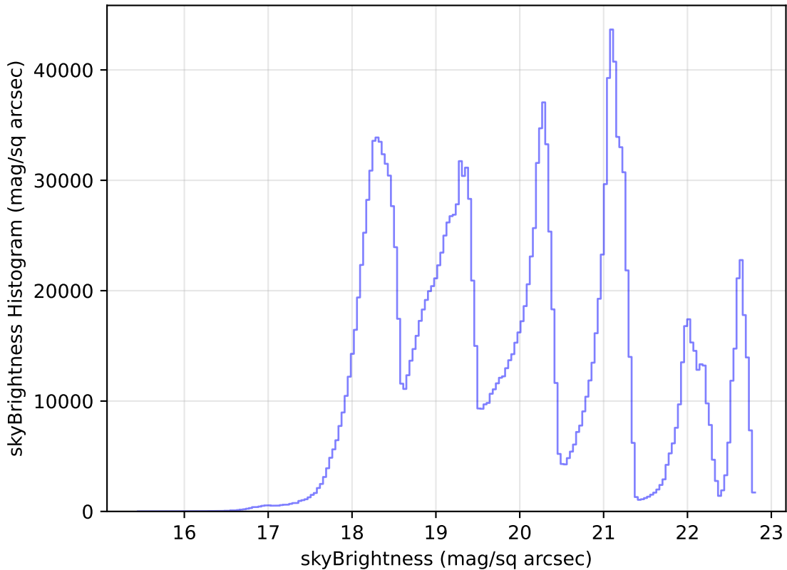
weather_cloudso14v3.4_10yrs WFD all bands: skyBrightness Histogram
