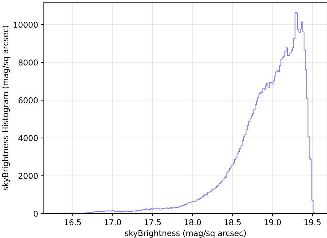
weather_cloudso14v3.4_10yrs All sky z band: skyBrightness Histogram
