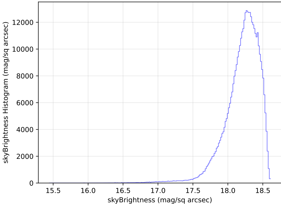
weather_cloudso14v3.4_10yrs All sky y band: skyBrightness Histogram
