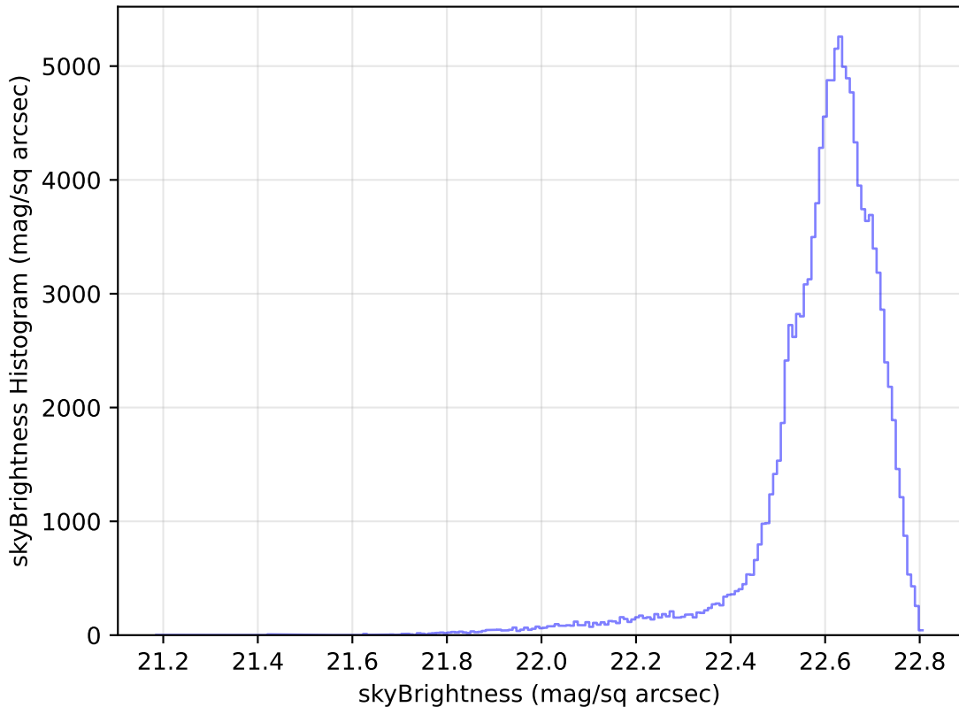
weather_cloudso14v3.4_10yrs All sky u band: skyBrightness Histogram
