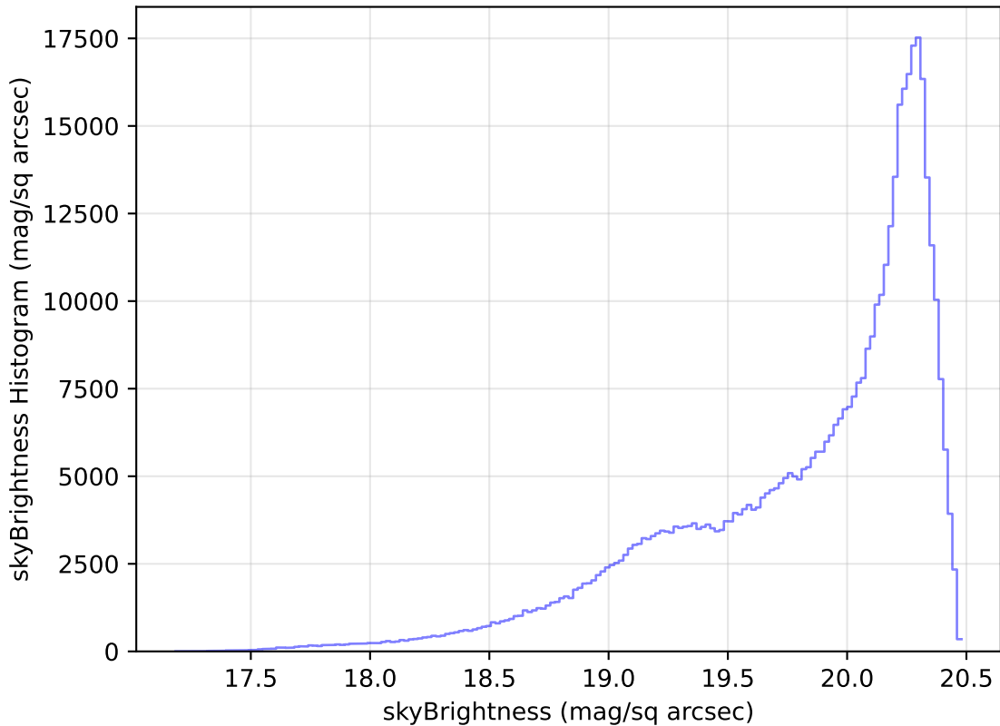
weather_cloudso14v3.4_10yrs All sky i band: skyBrightness Histogram
