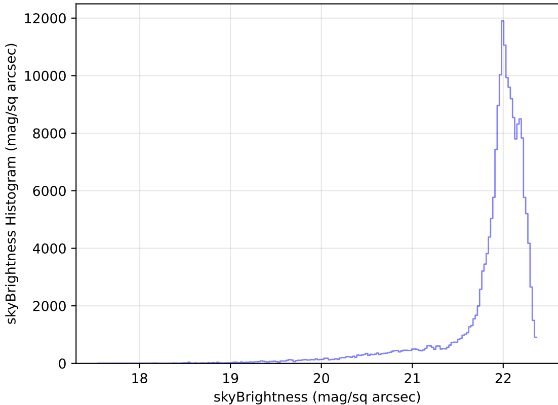
weather_cloudso14v3.4_10yrs All sky g band: skyBrightness Histogram
