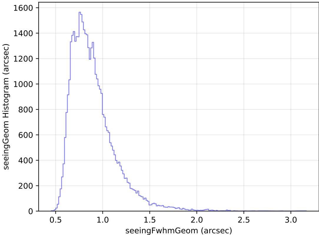
weather_cloudso14v3.4_10yrs Yr 1 z band: seeingGeom Histogram
